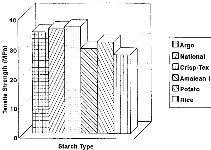
FIG. 2. Effect of starch type on tensile properties ( N = 5 ).
