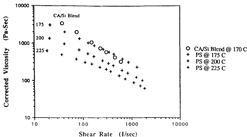
FIG. 3. Comparison of the rheology of cellulose acetate/Argo starch blends with polystyrene.
