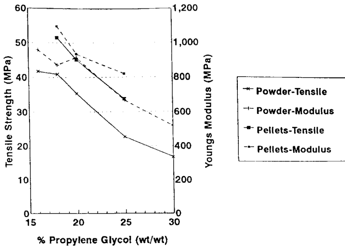
FIG. 1. Mechanical properties of cellulose acetate/propylene glycol tensile bars produced from powders and extruded pellets ( N = 5 ).
