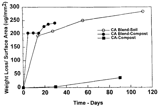
FIG. 5. Weight loss/surface area of cellulose acetate (2.5 DS) in compost and cellulose acetate/corn starch/propylene glycol blends in compost and soil.
